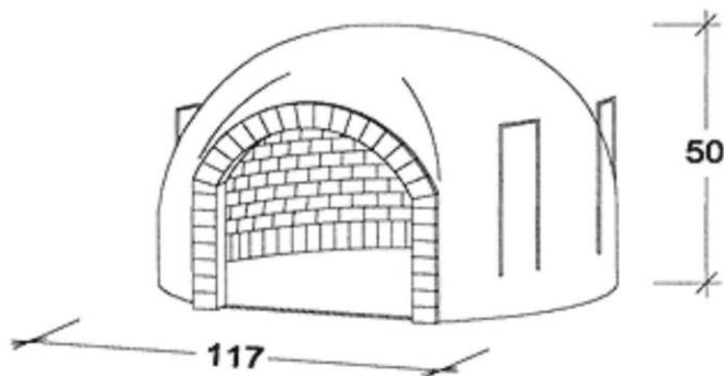
Artigiano100 footprint
