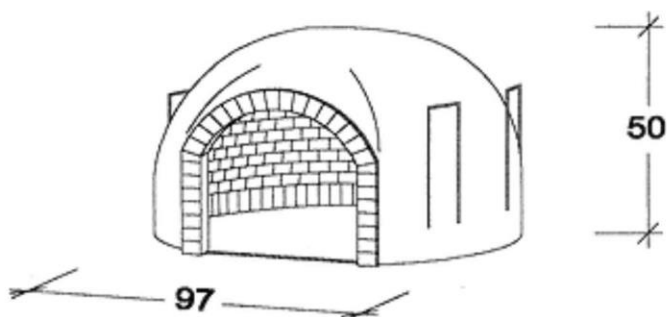
Artigiano80 footprint
