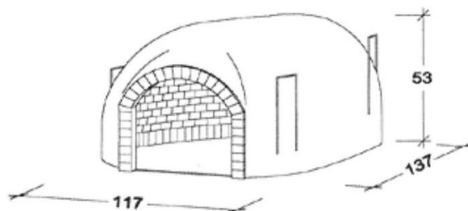
Artigiano120 footprint
