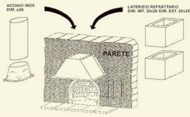
Vent installation
